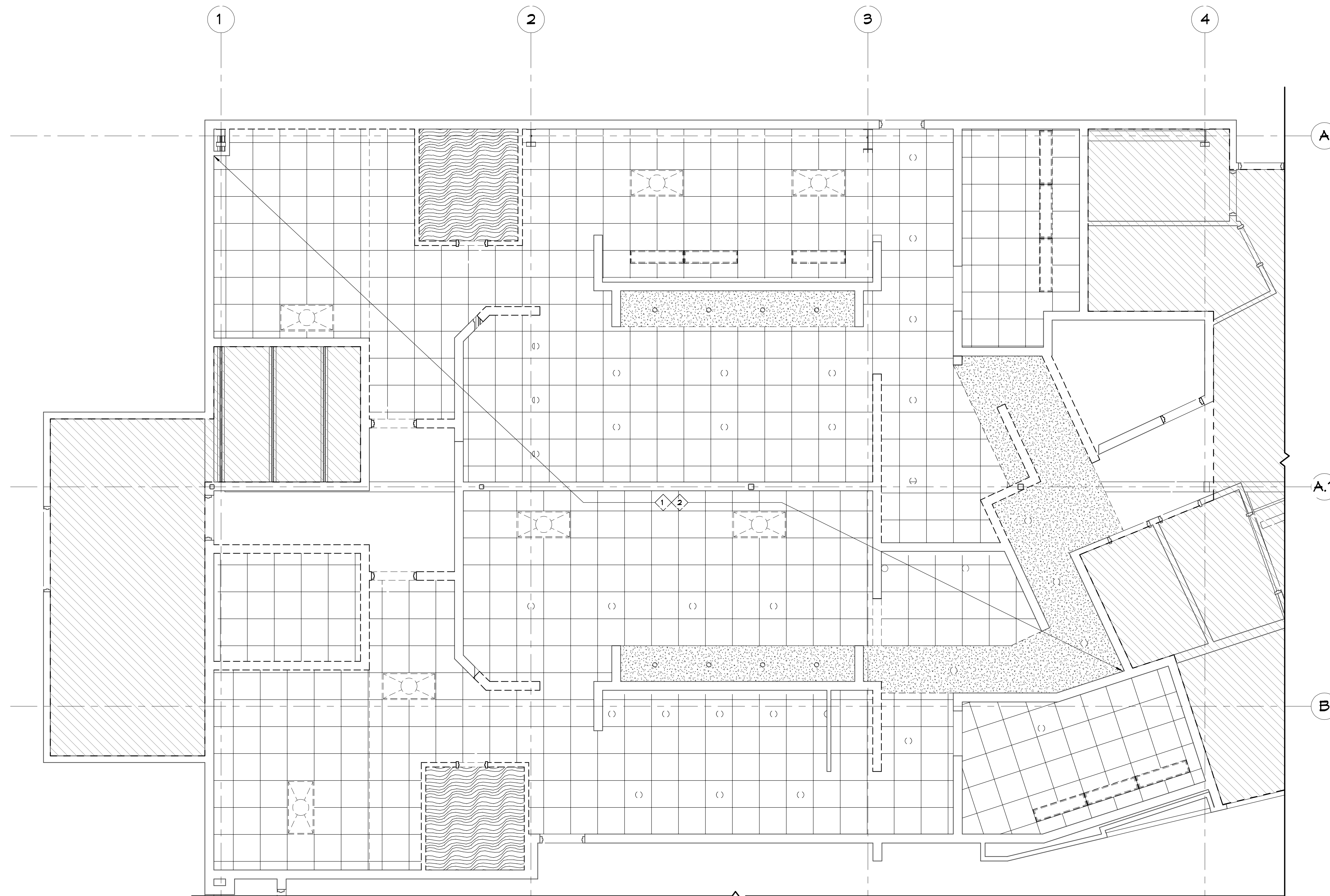
21ST FLOOR BLDG A DEMO REFLECTED CEILING PLAN SCALE: 1/4"=1'-0"
