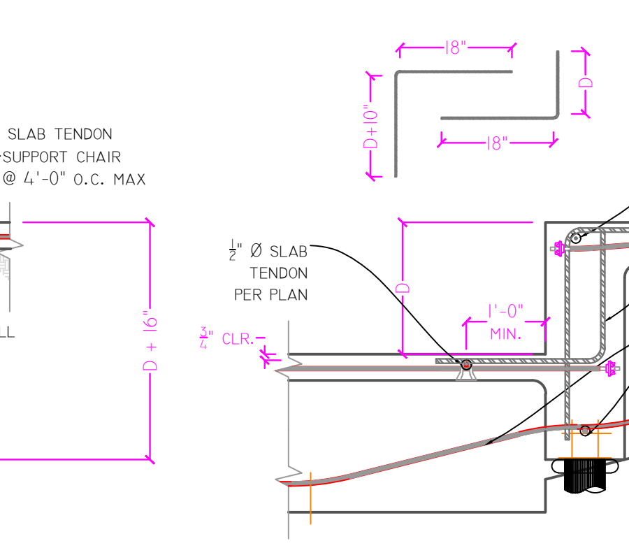
32 STOP-START AT BEAM TRANSITION FOR D <= 36" w/PILES Scale: 3/4" = 1'-0"
