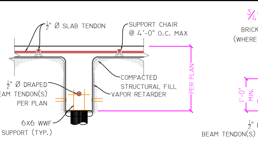
22 INTERIOR BEAM SECTION w/PILES Scale: 3/4" = 1'-0"
