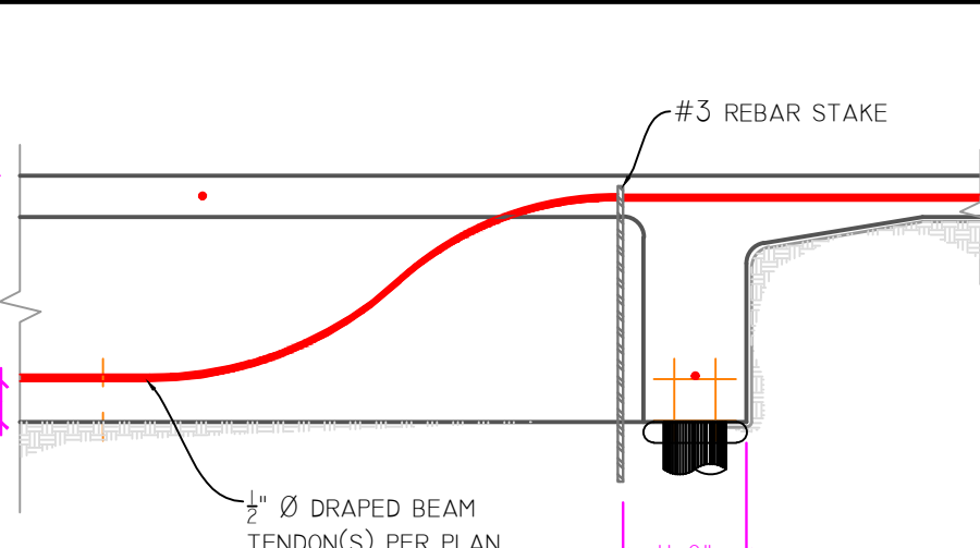
25 INTERIOR BEAM TENDON TRANSITION w/PILES Scale: 3/4" = 1'-0"
