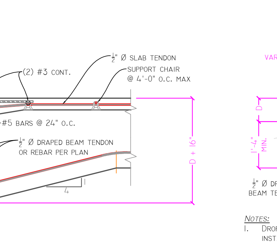
33 EXTERIOR BEAM AT DROP BRICK LEDGE <= 8" w/PILES Scale: 3/4" = 1'-0"
