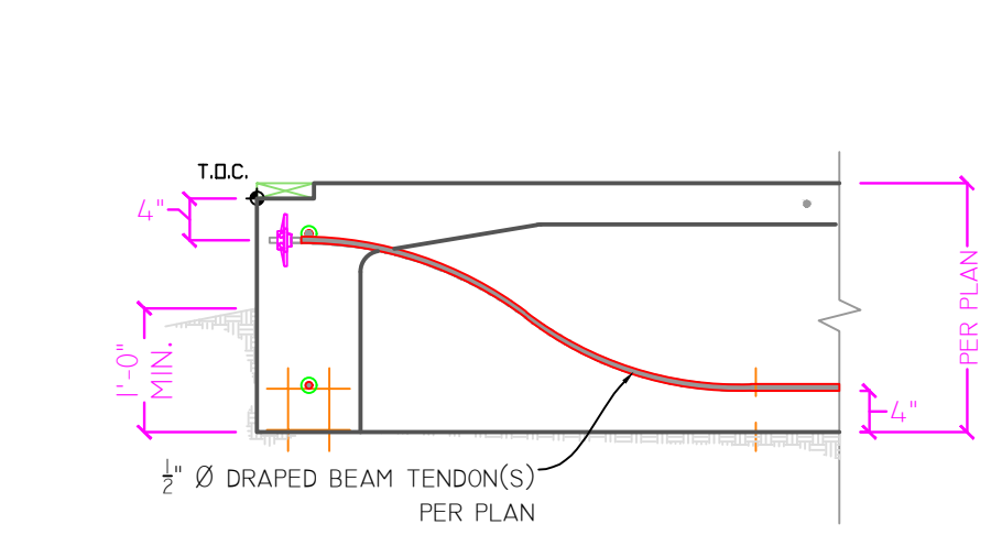
30 TYPICAL TENDON DRAPE AT EXT. BEAM INTERSECTION w/PILES Scale: 3/4" = 1'-0"
