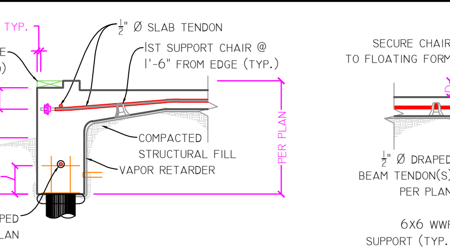
23 EXTERIOR BEAM SECTION AT GARAGE w/PILES Scale: 3/4" = 1'-0"
