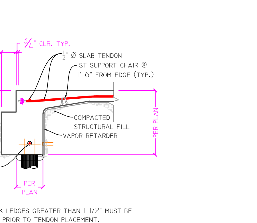
34 EXTERIOR BEAM AT DROP BRICK LEDGE <= 36" w/PILES Scale: 3/4" = 1'-0"
