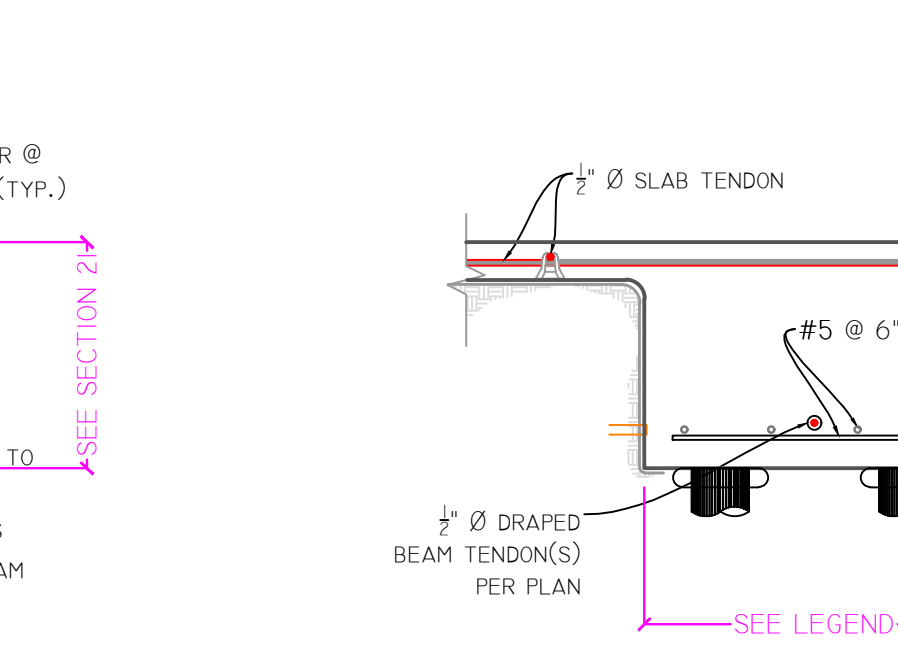
38 BEAM AT EXISTING FOUNDATION w/PILES Scale: 3/4" = 1'-0"
