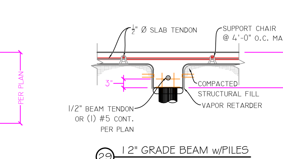
29 12" GRADE BEAM w/PILES Scale: 3/4" = 1'-0"
