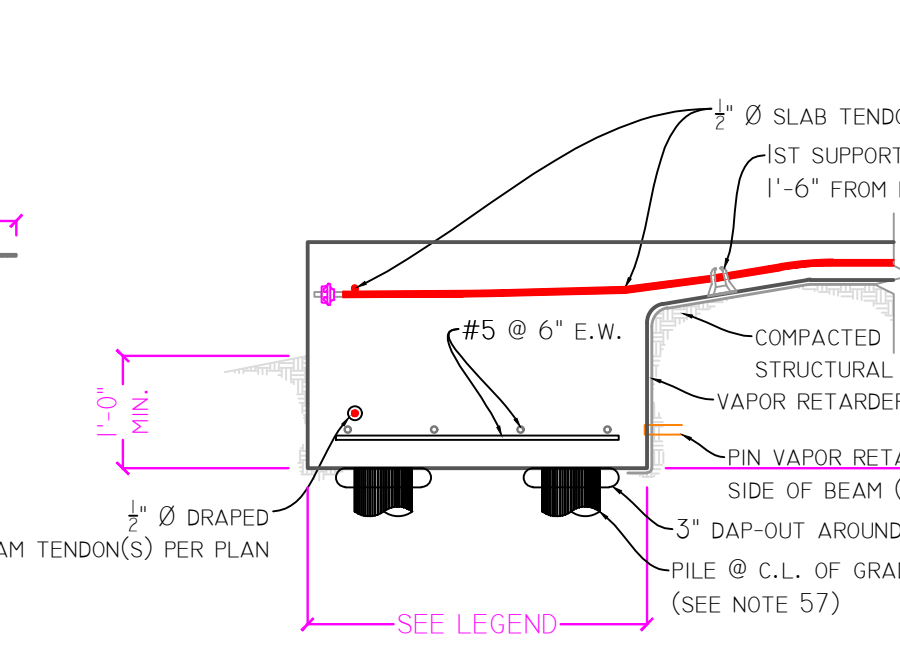
37 INTERIOR COLUMN FOOTING w/PILES Scale: 3/4" = 1'-0"
