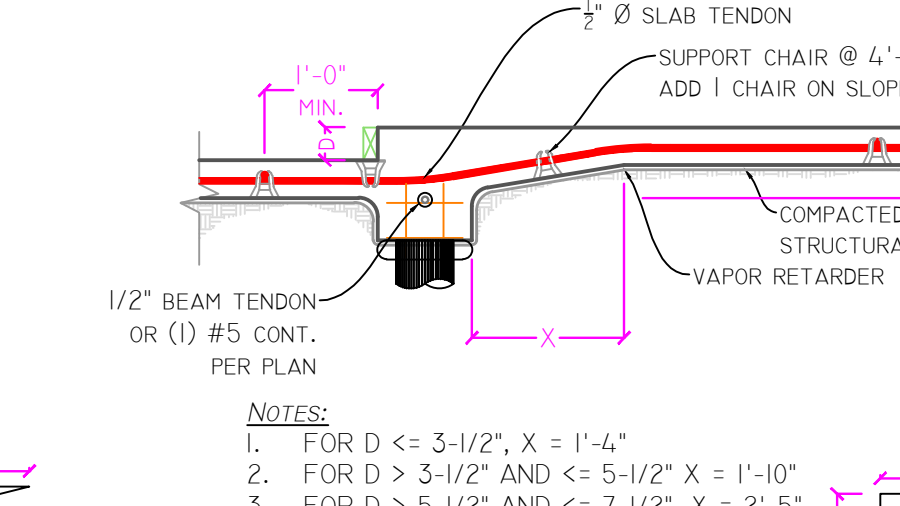
27 THICKENED SLAB TENDON TRANSITION w/PILES Scale: 3/4" = 1'-0"
