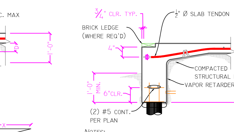
28 EXTERIOR BEAM SECTION w/ REBAR & PILES Scale: 3/4" = 1'-0"
