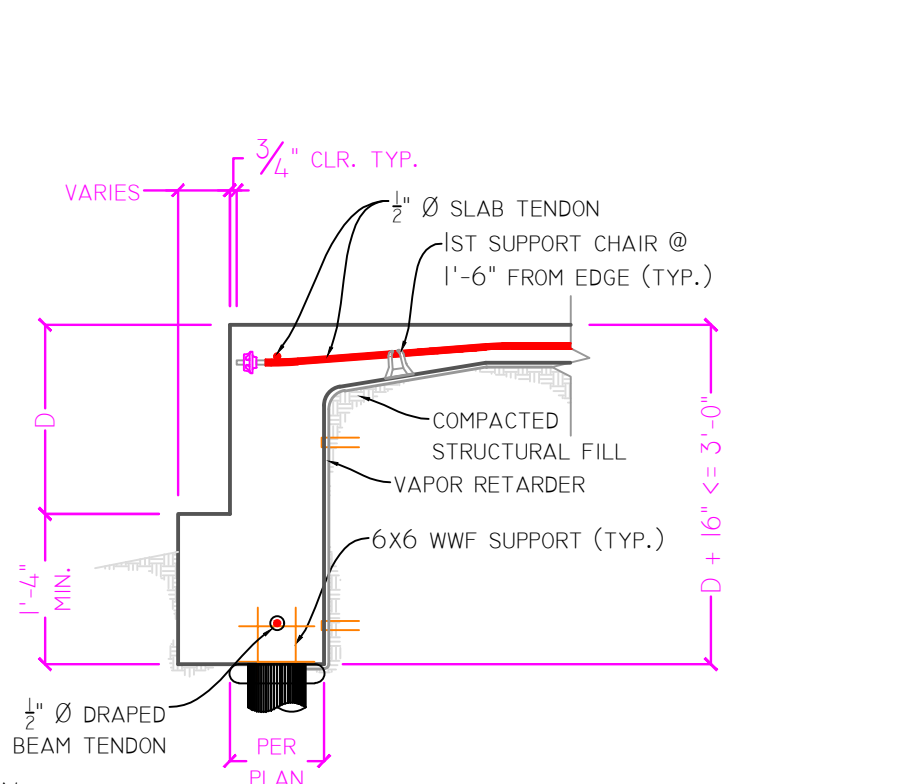
35 BEAM AT EXISTING FOUNDATION w/PILES Scale: 3/4" = 1'-0"
