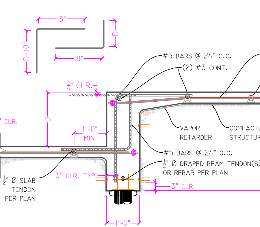
31 STOP-START FOR D <= 36" w/PILES Scale: 3/4" = 1'-0"
