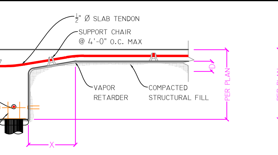
24 INTERIOR BEAM TENDON TRANSITION w/PILES Scale: 3/4" = 1'-0"
