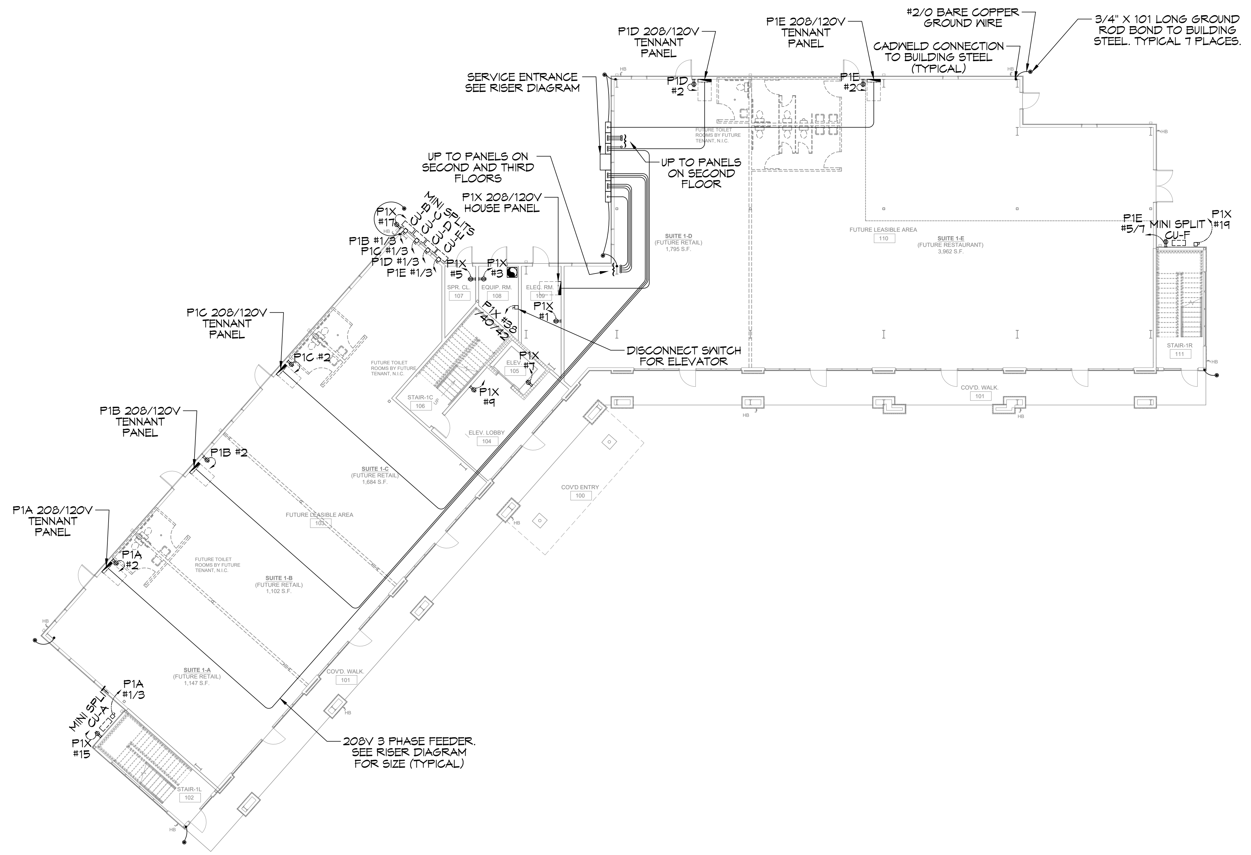
27 FIRST FLOOR POWER PLAN SCALE: 3/32"=1'-0"
