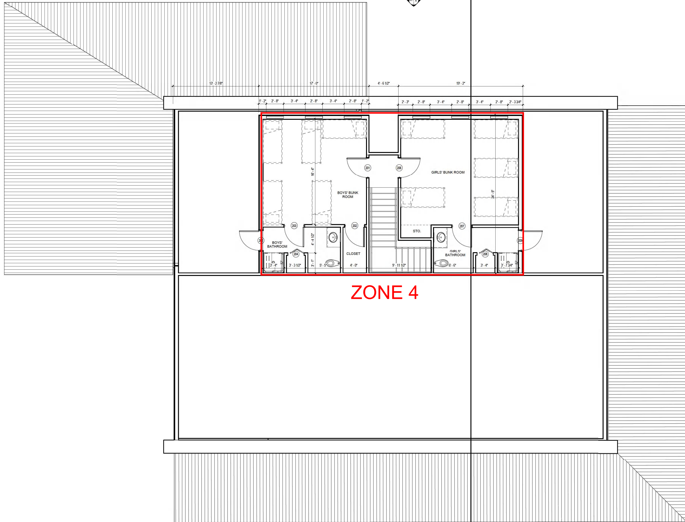
1 LOFT PLAN A2.2 1/4" = 1'-0"
