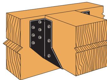
Typical OHU Installation
