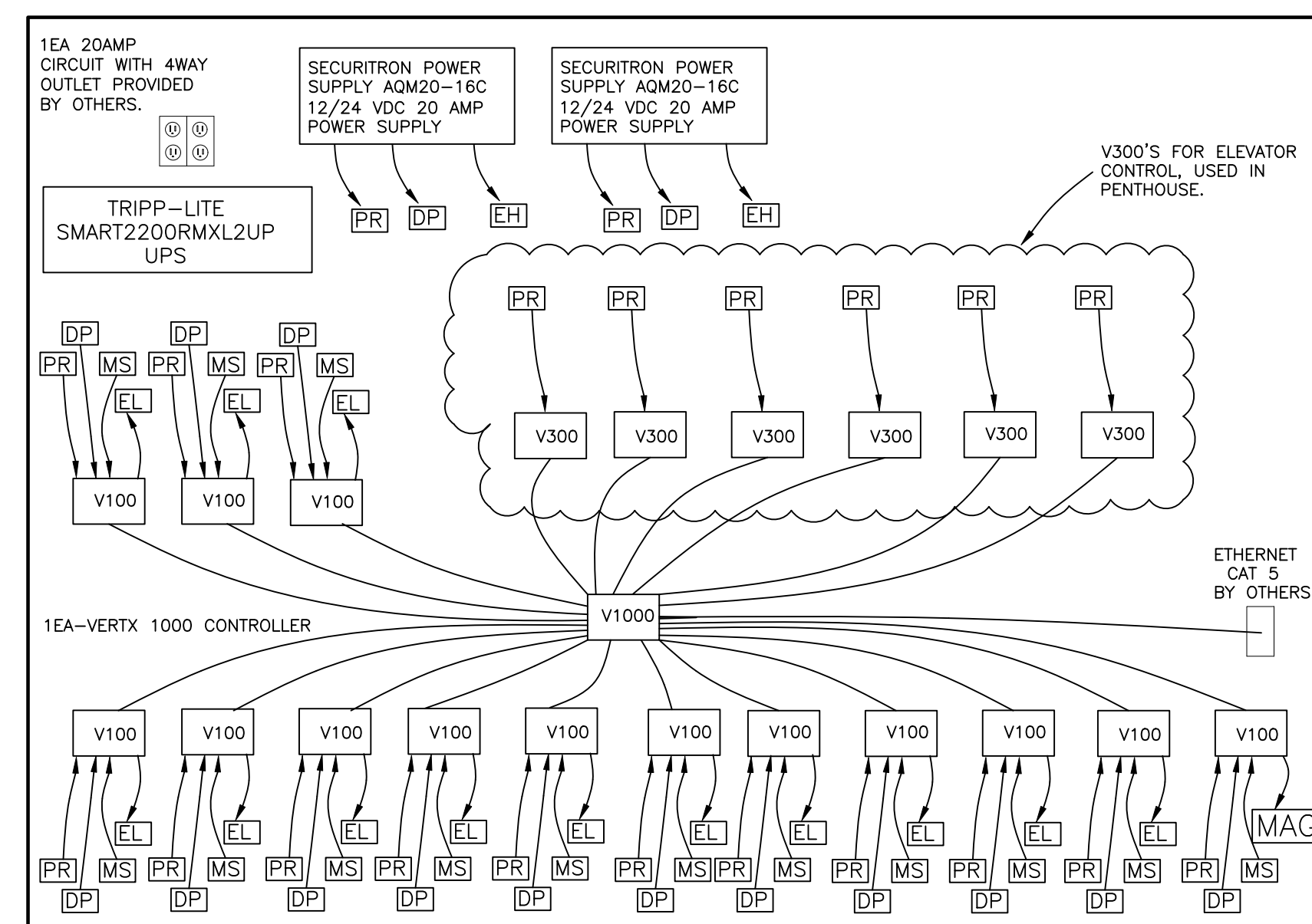
5th FLOOR 5241 EQUIPMENT ELEVATION
