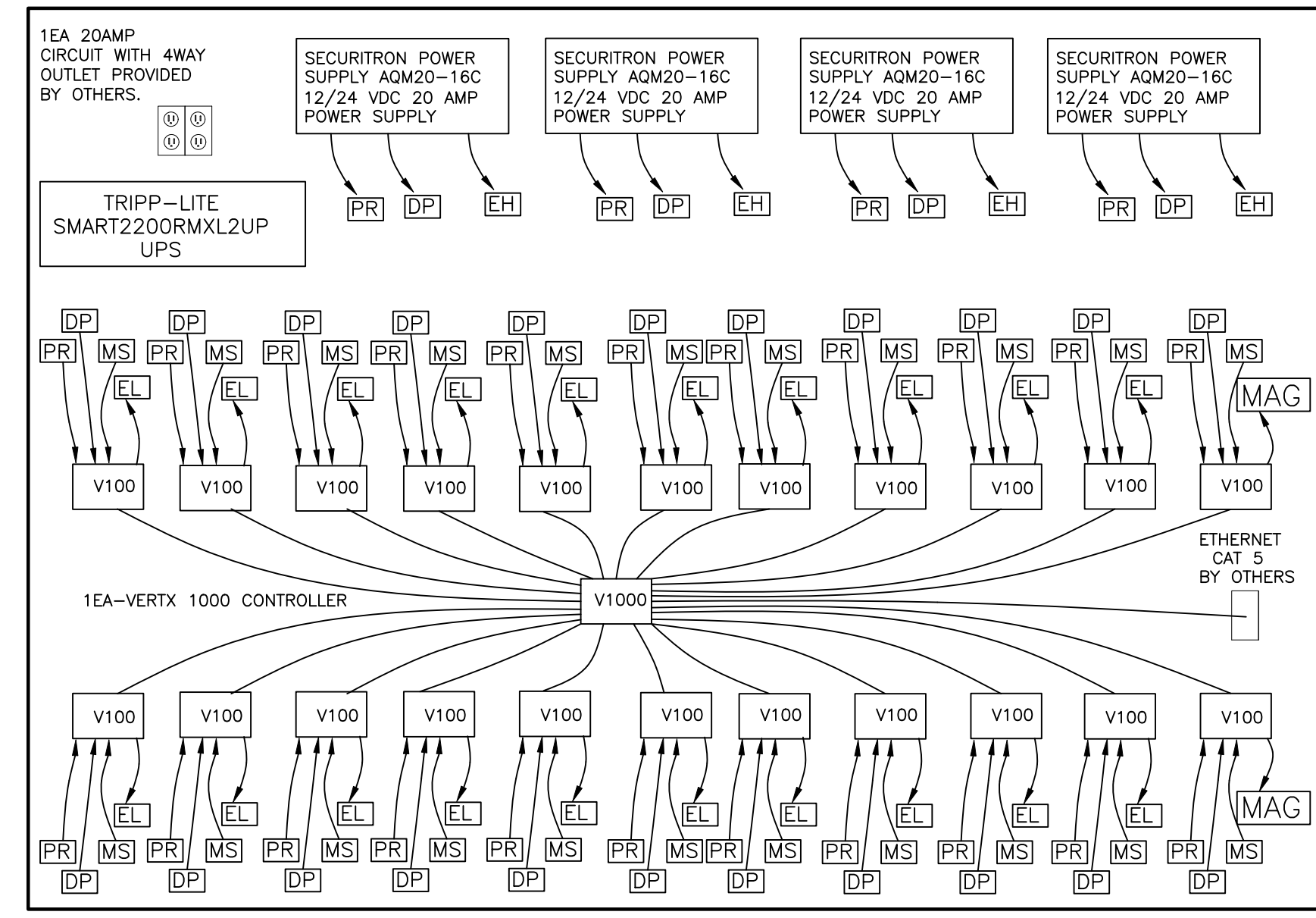
1st FLOOR 1323 EQUIPMENT ELEVATION
