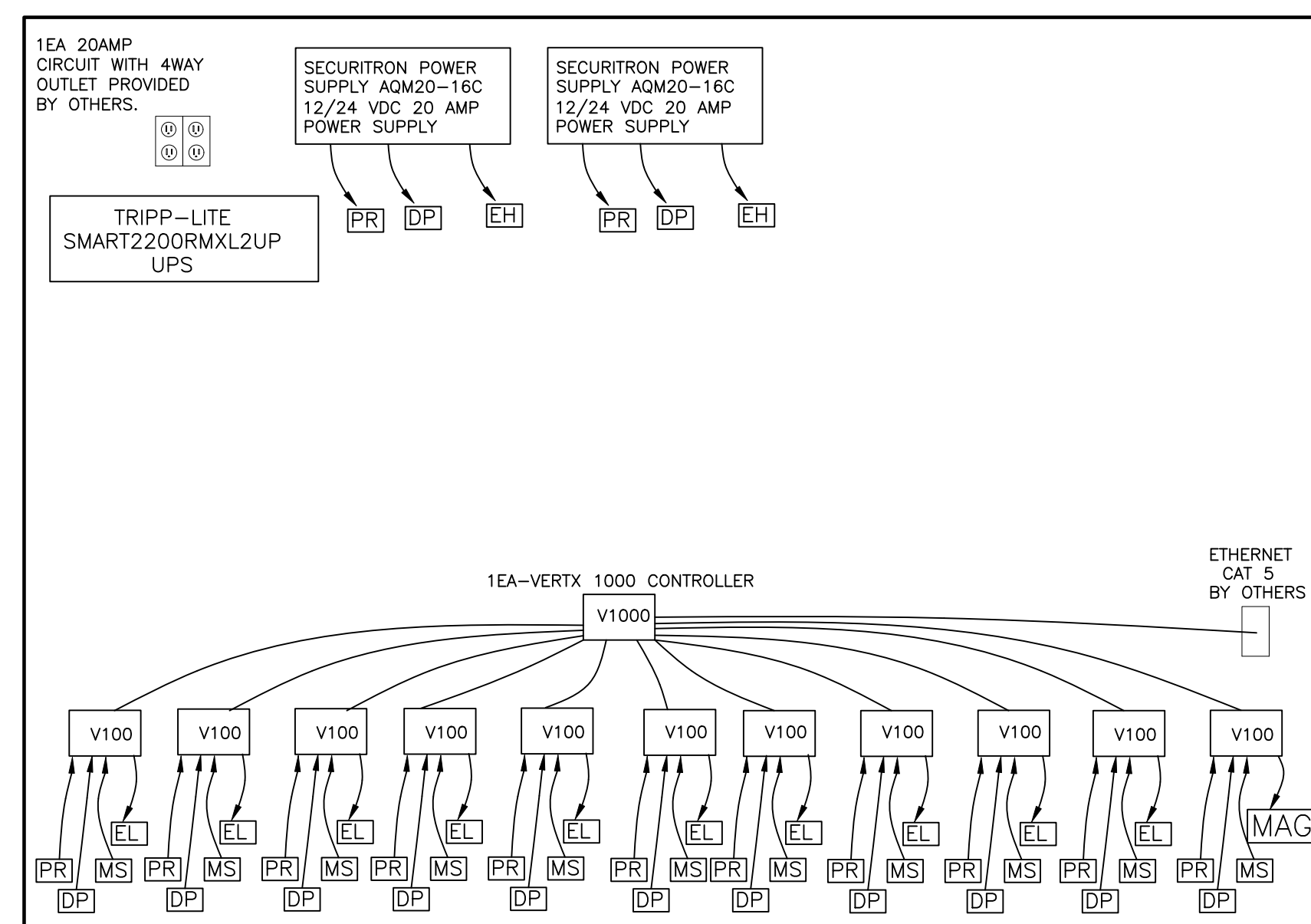
4th FLOOR 4231 EQUIPMENT ELEVATION
